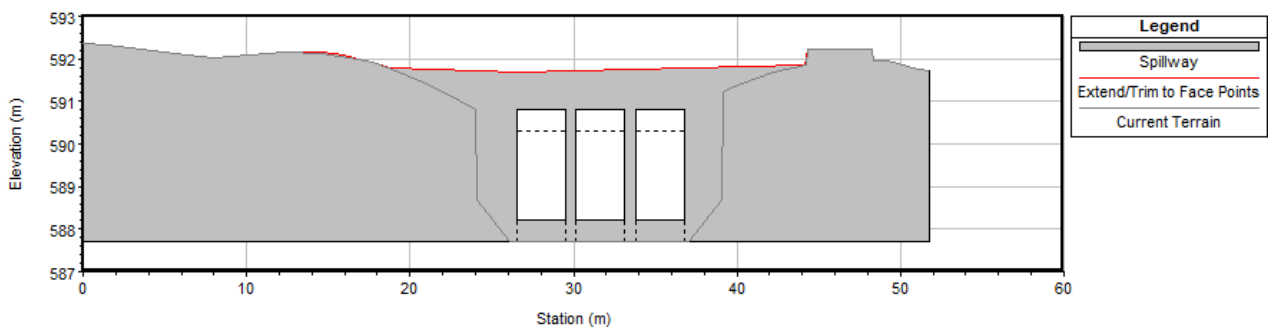
Image 5-2: Screenshot of the HEC-RAS 6.3.1 graphical interface, with the introduction of the geometric characteristics of the spans of a technical work, upstream to downstream view.
