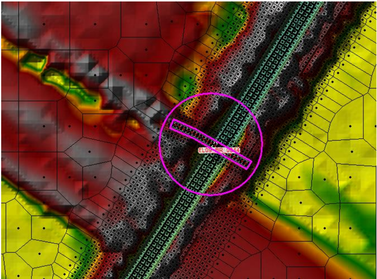
Image 5-1: Screenshot of the HEC-RAS 6.3.1 graphical interface, with the DTM in the background, the two-dimensional solution grid, and an engineering structure perpendicular to the watercourse flow.
