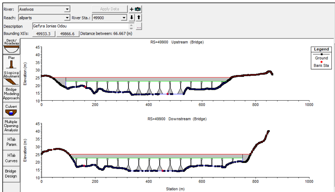
Figure 5-2: Snapshot of HEC-RAS 6.4.1 GUI, with the input of the geometric characteristics of the openings of the technical project, upstream to downstream view
