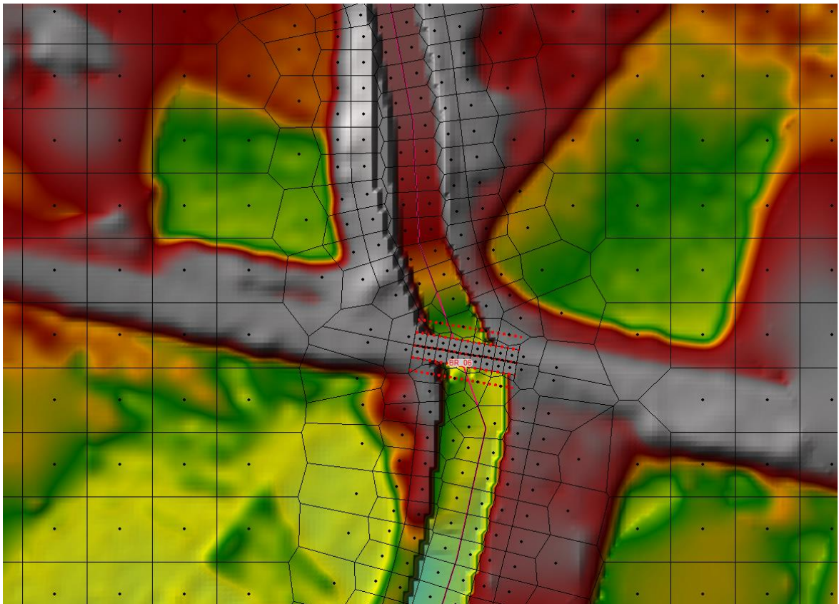
Figure 5-1: Snapshot of HEC-RAS 6.4.1 graphical environment, with the DEM background, the 2D solution grid and technical project perpendicular to the stream
